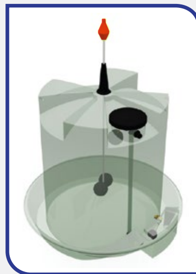
DP640 10,000L TANK & TROUGH COMBO WITH LEVEL INDICATOR
